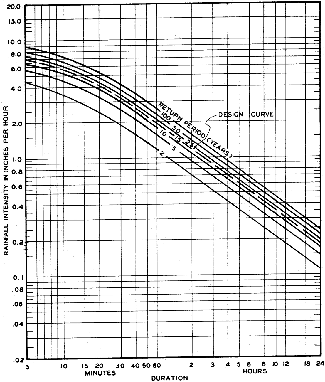
RAINFALL INTENSITY - DURATION - FREQUENCY CURVES
