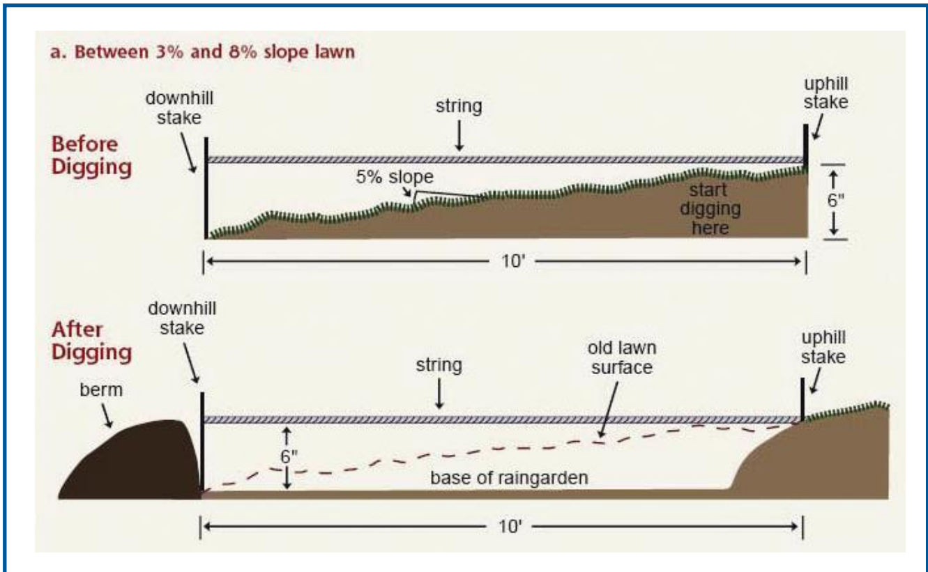
Figure 16 – Determining rain garden depth based on slope of the lawn (Rain Garden Initiative, Toledo-Lucas County)
