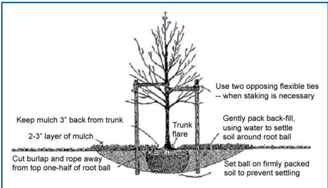
Figure 8 – Properly planted and staked tree
