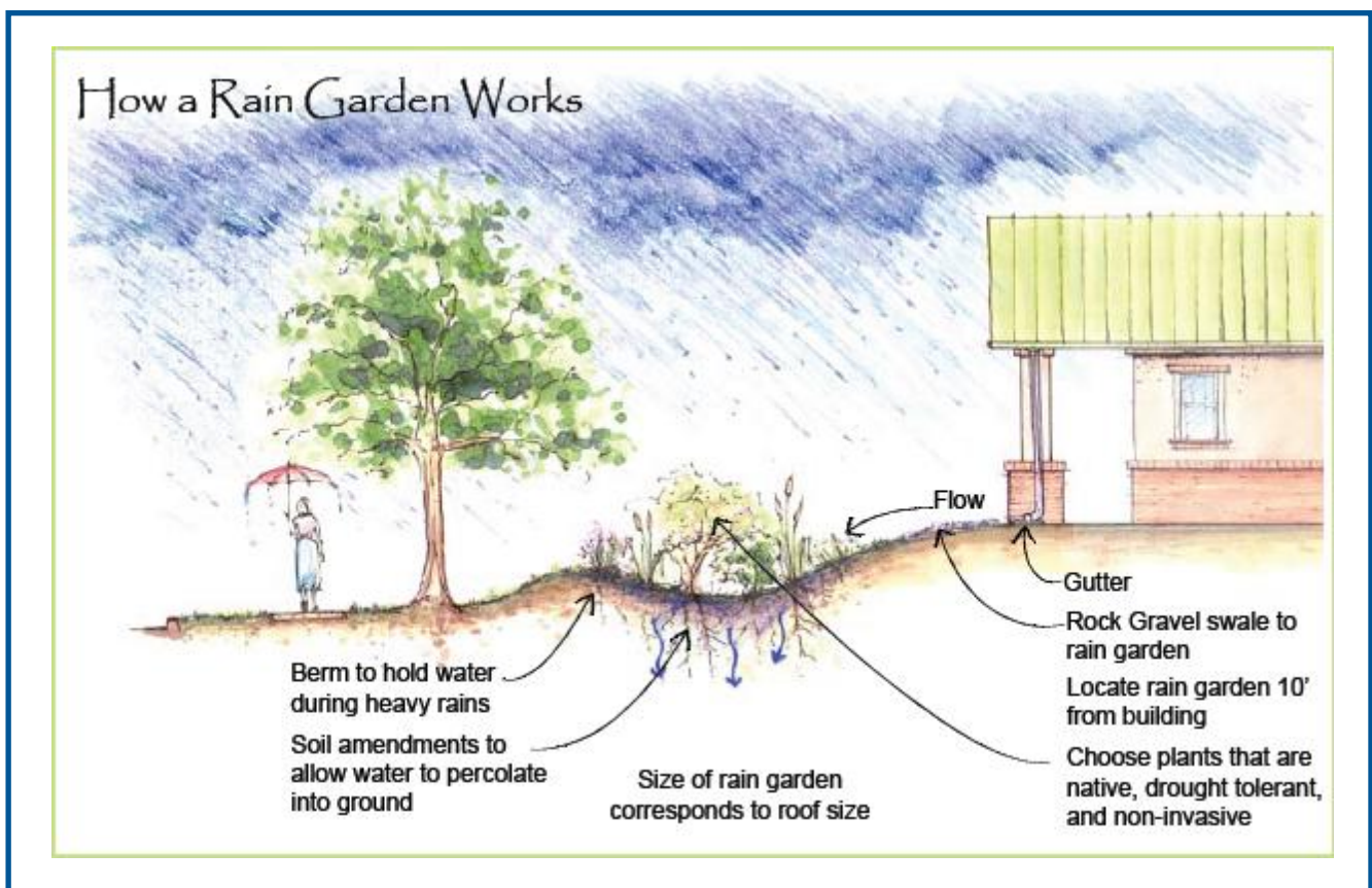
Figure 15 – How a rain garden works (Rain Garden Initiative, Toledo-Lucas County)
