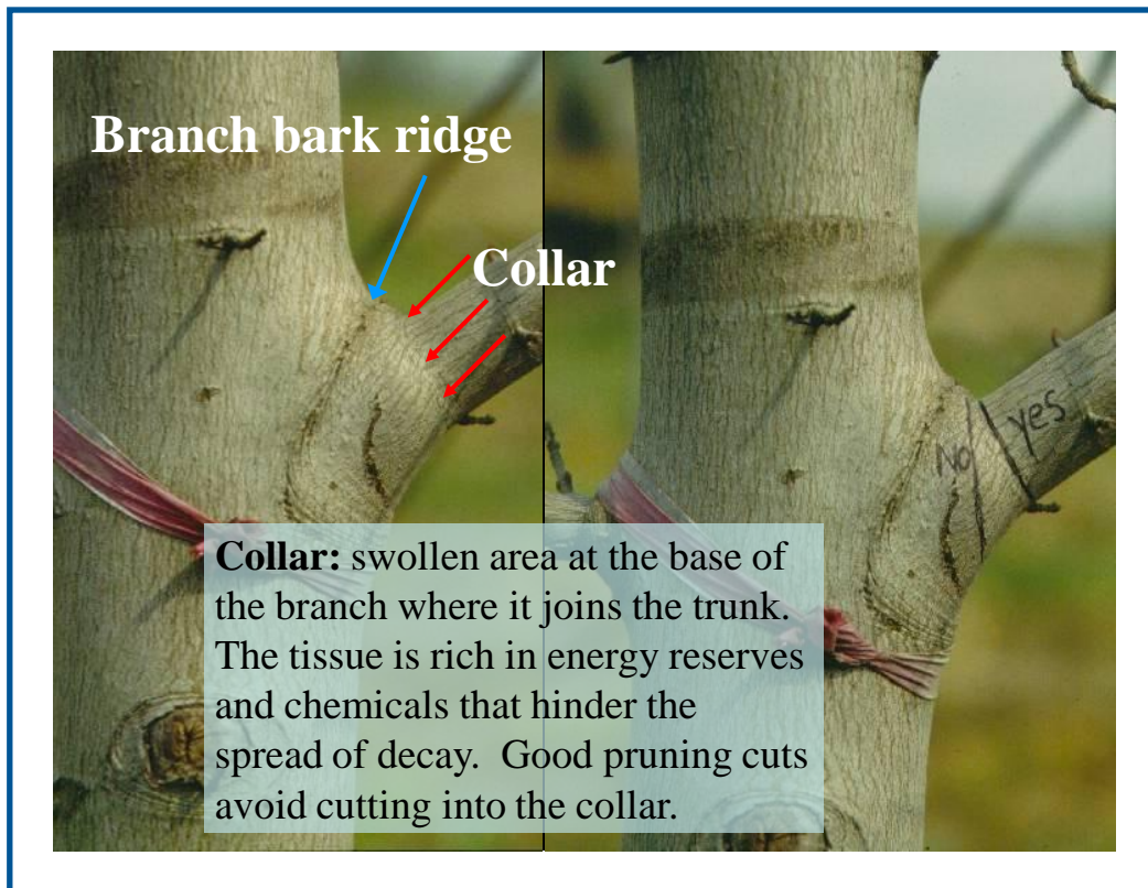
Figure 12 – Proper pruning cuts should be made outside of the branch collar (Dr. Edward Gilman, University of Florida)
